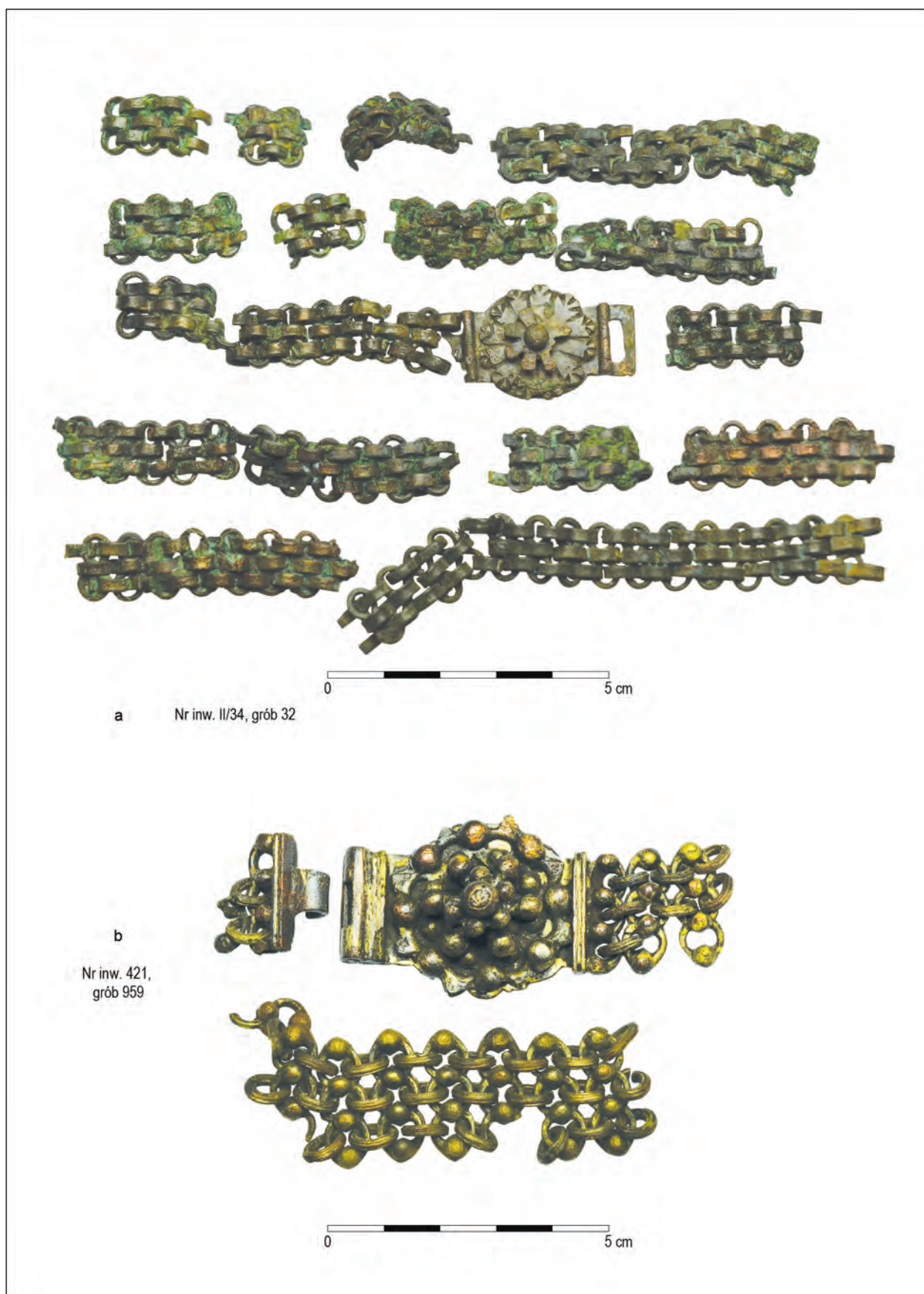
Tabl. 1. Wrocław, cmentarz Salwatora. Pasy ogniwkowe z klamrami. Fot. J. Wojcieszak Table 1. Wrocław, cemetery of Our Saviour. Ring belts with buckles. Photo by J. Wojcieszak
